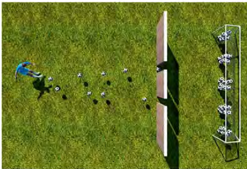
Buckyball Soccer When molecular soccer balls are fired at slits in a screen, the resulting pattern reflects unfamiliar quantum laws.
